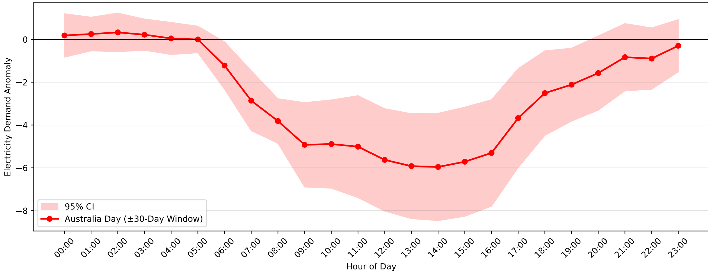
Newcastle Cbd Demand Anomaly: Australia Day (2004-2017, \pm 30 -Day Window)
